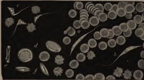
FIG. 135.—MONADS IN RAT'S BLOOD, \times 1200 .
